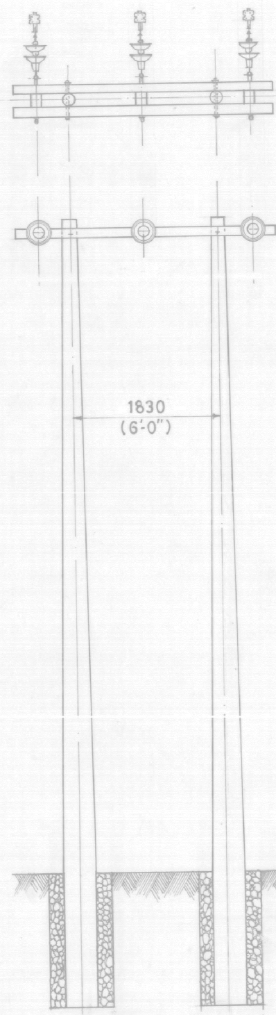
ELEVATION "A" 'H' POLE
