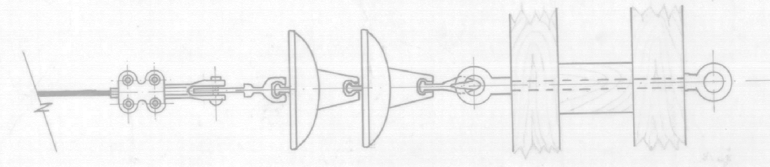
ASSEMBLY OF STRAIN TYPE INSULATORS TOP VIEW
