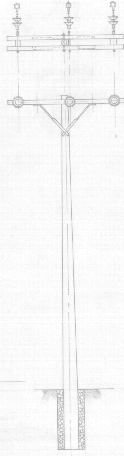
ELEVATION "B" SINGLE POLE
